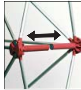
1/ When erected, the aluminium structure is automatically and instantly held into position with magnetic locking pins .
